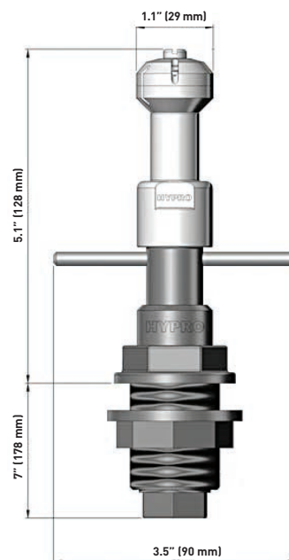
ProClean container nozzle with valve
